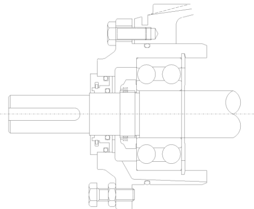
Frame 1 to 4 proprietary labyrinth/face seals (where fitted)
